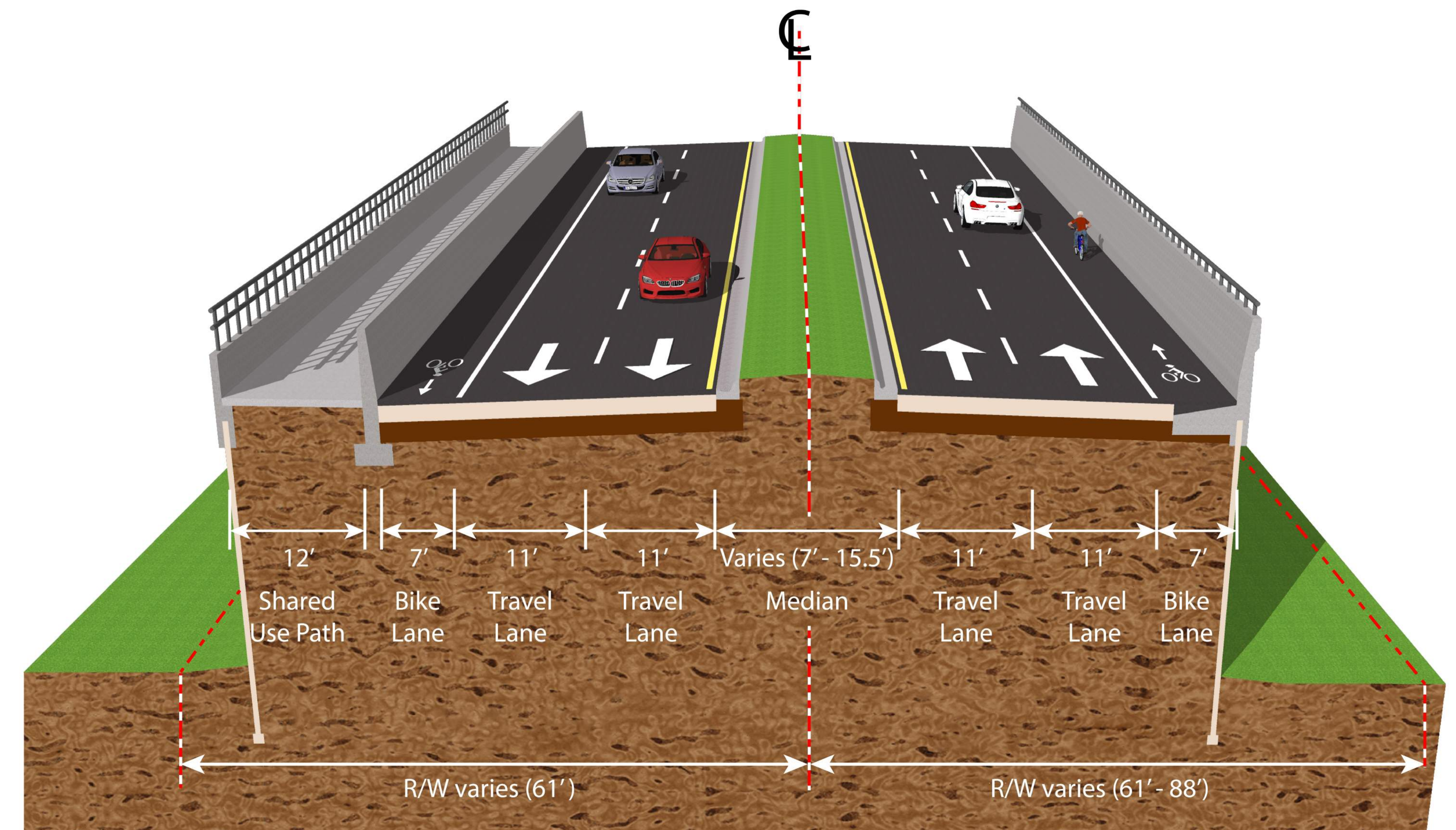
New North Sarasota Multimodal Connector Roadway Four-Lane Elevated Typical Section
