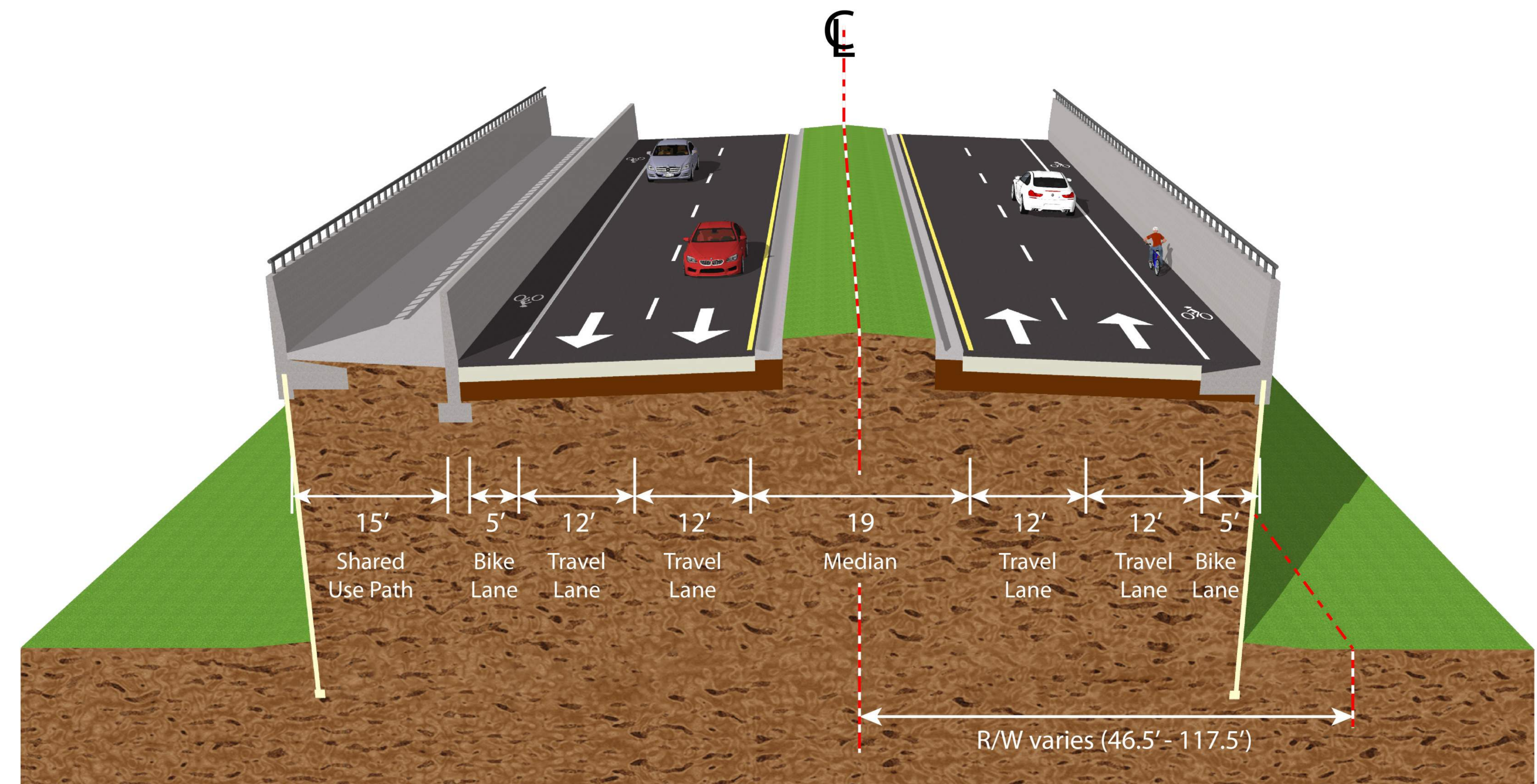
Reconstructed North Cattlemen Road Four-Lane Elevated Typical Section
