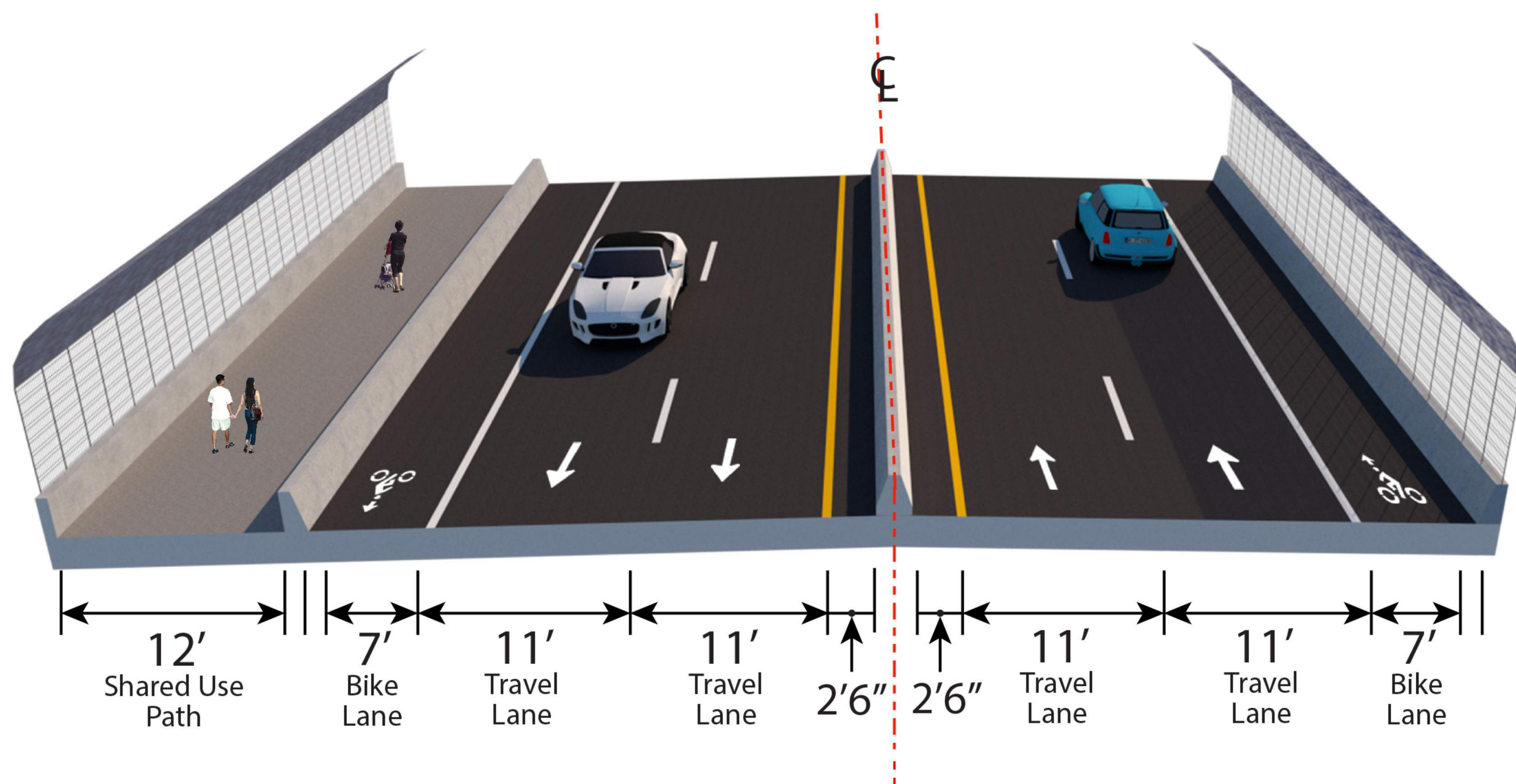
New North Sarasota Multimodal Connector Roadway Four-Lane Bridge Typical Section
